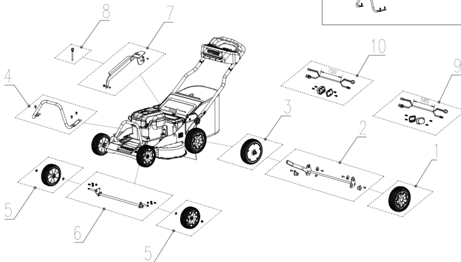
2519207RU—Exploded view
