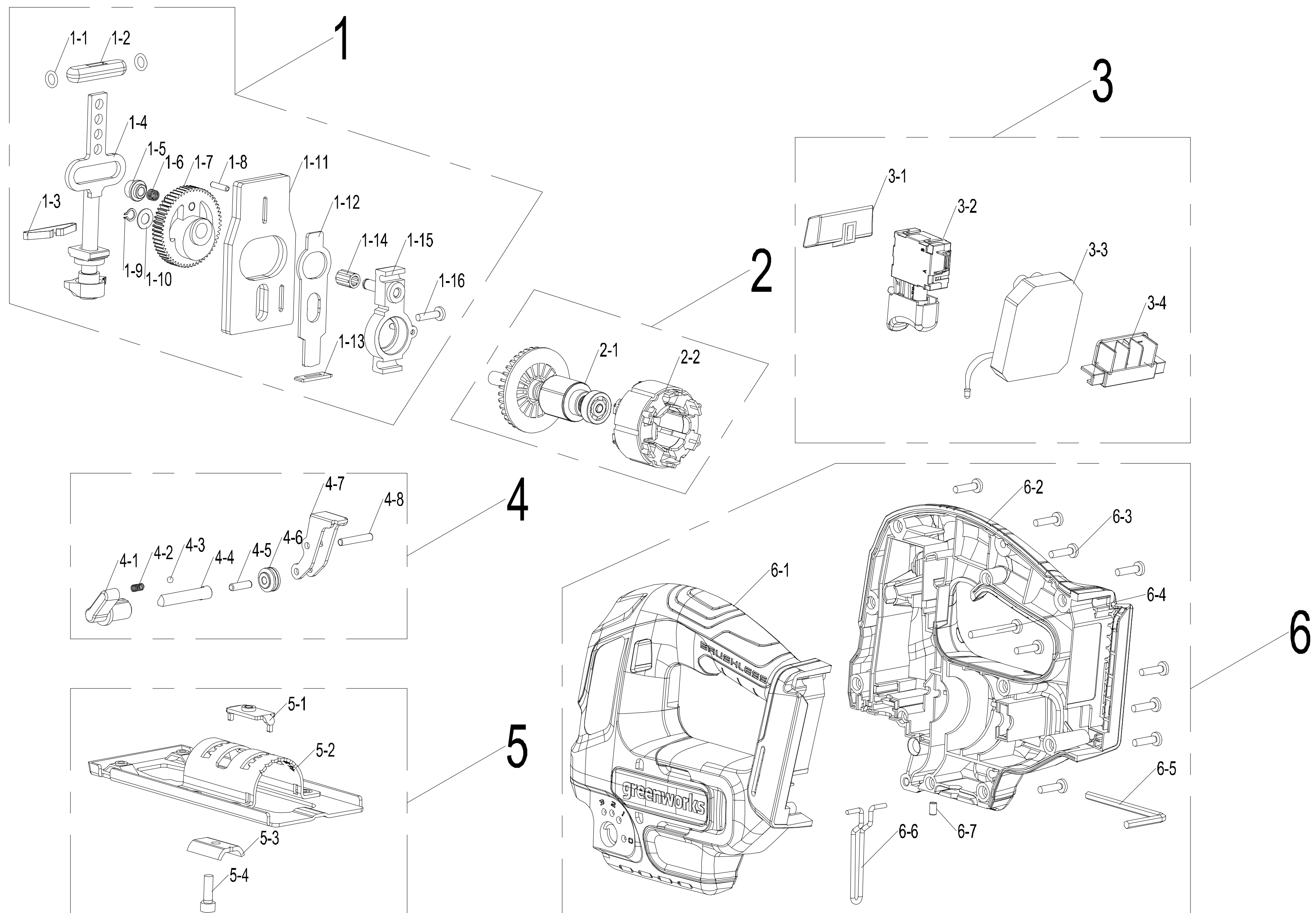
3601707RU-Exploded view
